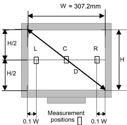
FIG. 3 Luminance Uniformity-Angular Dependent(TCO 99)
