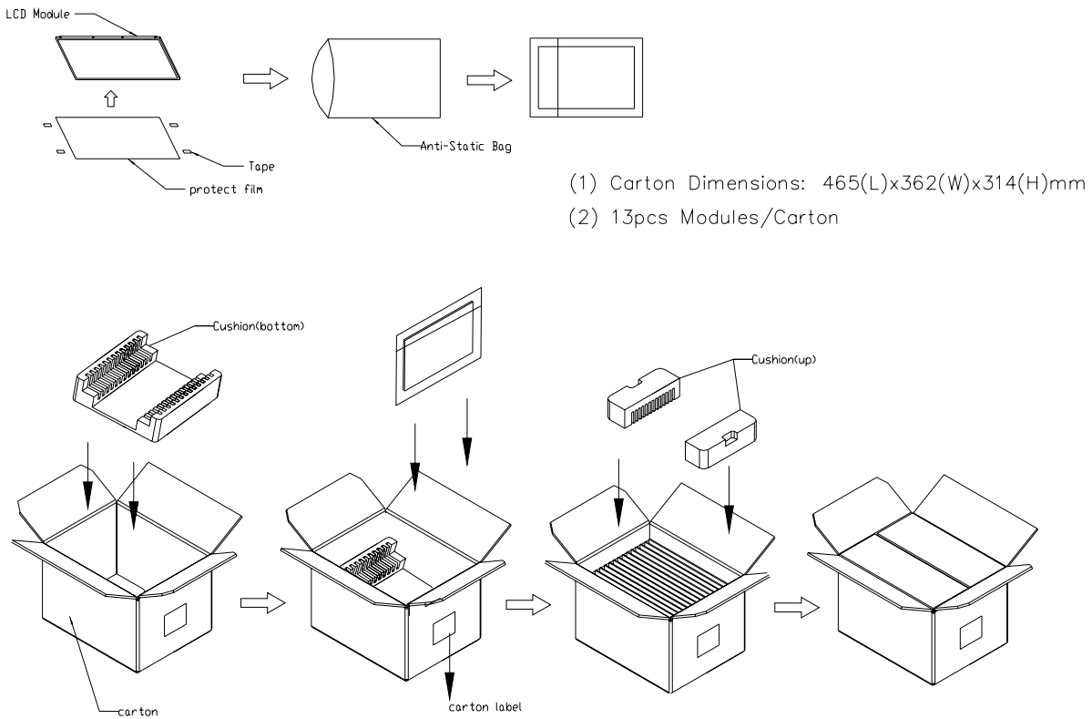
Figure. 9-1 Packing method
