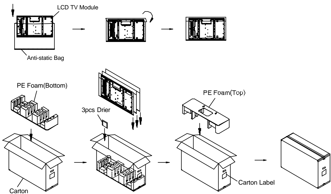
Figure.9-1 packing method
