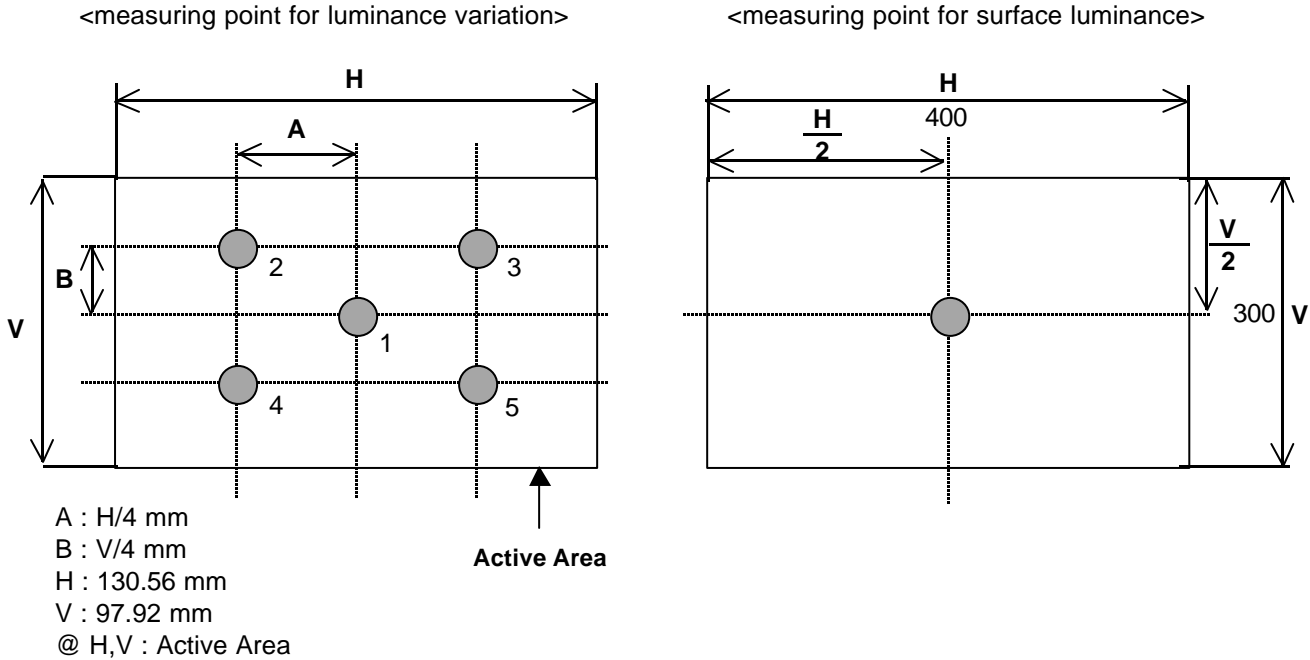
FIG. 2 Luminance
