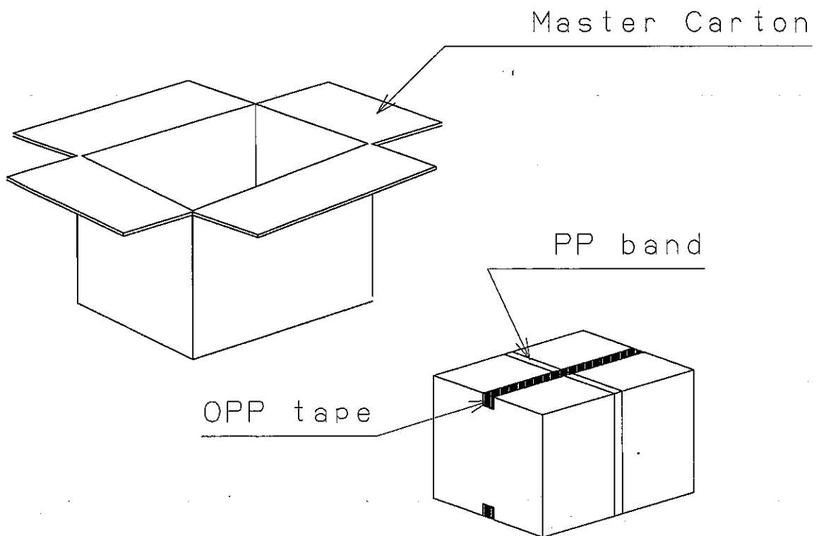
Fig.1 Packing Form (LQ0DZA0051)
